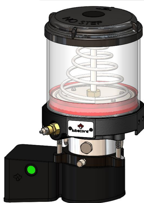
Figure 1 4kg Pump shown with 58.497 Reservoir
